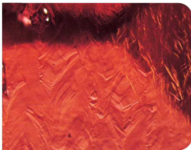
Figure 6. The most distinctive visual feature of the hydrothermal synthetic red beryls examined was chevron-like internal growth zoning. From observations in the original crystals, we know that this zoning is oriented along the direction of crystal growth at a high, oblique angle to the plane of the seed plate. Photomicrographs by James Shigley; left—magnified 3 \times , right—magnified 9 \times .
