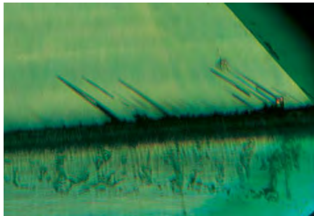
Figure 14. The third type of elongated inclusion seen in the Chinese samples consists of needle-like tubes with an orientation almost perpendicular to the surface of the synthetic emerald seed (seen at the bottom here). On the other side of this boundary, in the synthetic emerald overgrowth, the cone-shaped spicules are elongated parallel to the c-axis. They start at the seed or at a short distance from the seed, and are often associated with tiny birefringent crystals that are in contact with the seed. (Note that the inclusion above the spicule on the right is not directly related to the spicule.) Immersion, crossed polarizers, magnified 80 \times .
