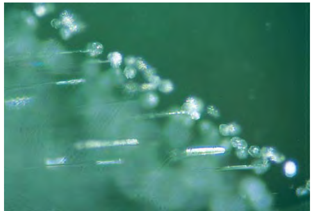
Figure 15. Micro-Raman analysis revealed that the tiny crystals at the broad ends of the numerous one- and two-phase cone-shaped spicules in the Chinese hydrothermal synthetic emeralds were chrysoberyl. Renishaw Raman microscope, magnified 200 \times .
